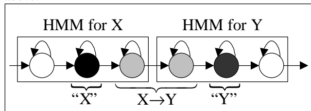
Figure 1. Motivation for 3-state HMM framework. Core states of phones model the canonical phone itself and are not highly affected by context. Remaining states model the context-dependent transition from phone to phone.
